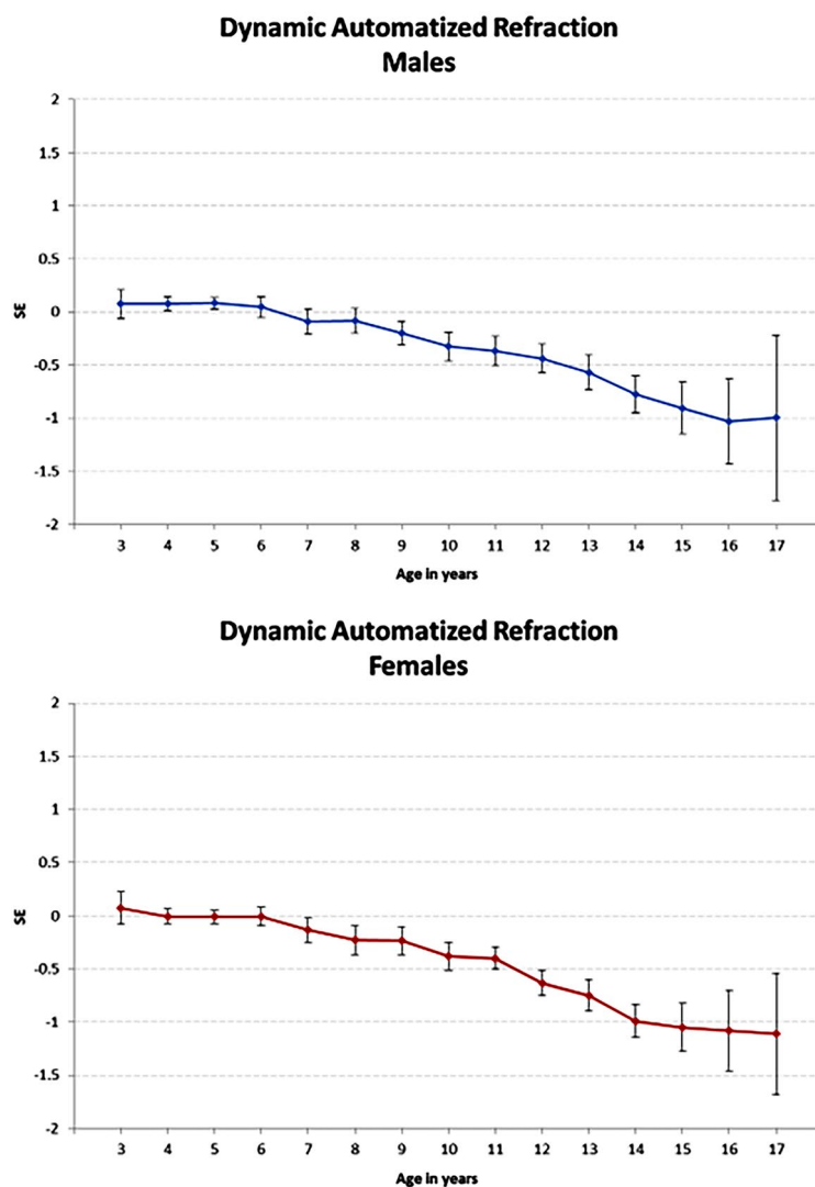
Fig. 2 Mean dynamic automatized refraction in spherical equivalent (SE) according to sex and age. Error bars show respective standard errors
